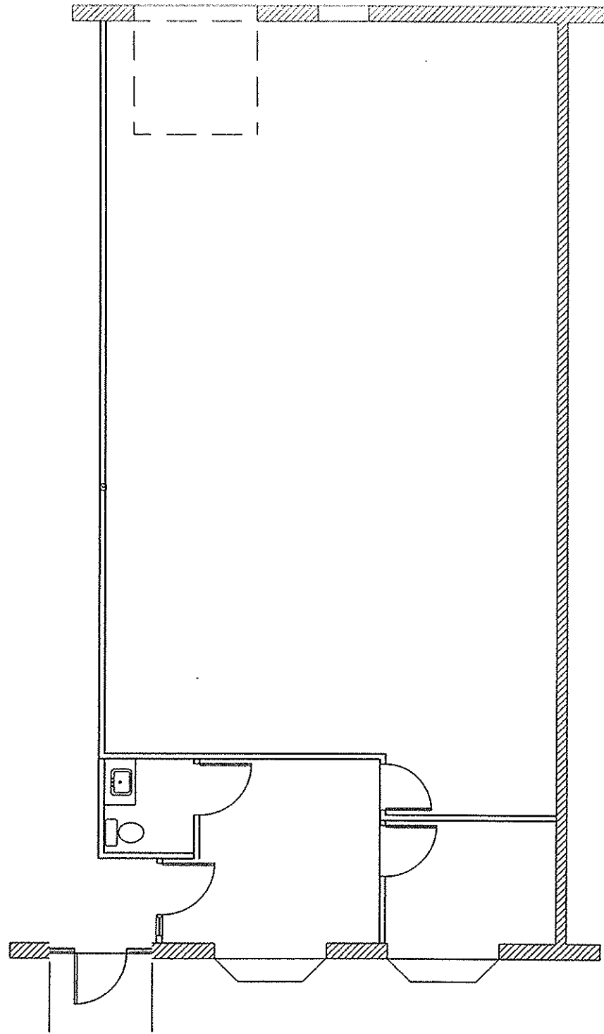
SUITE 219 1,860SF
